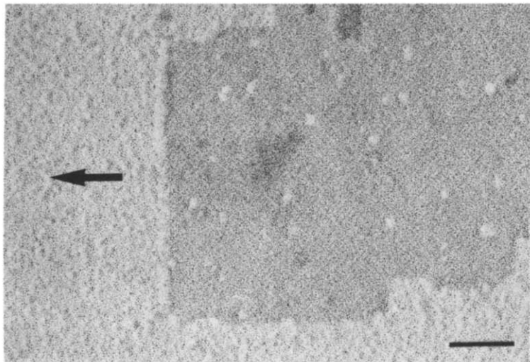
Fig. 2. NADH:Q oxidoreductase crystal, slightly negatively stained with uranyl acetate and shadowed with platinum from an angle of 26°. The direction of shadowing is indicated by the arrow. The bar represents 100 nm.
